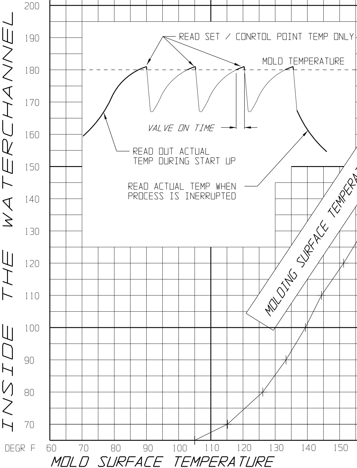
TEMPERATURE RELATIONSHIP DWG. NO. IWP-1820-A
