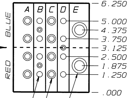
MANIFOLD HOLE PATTERN TOP VIEW (UNFOLDED)
