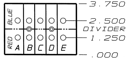
MANIFOLD HOLE PATTERN TOP VIEW (UNFOLDED)
