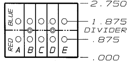
MANIFOLD HOLE PATTERN TOP VIEW (UNFOLDED)
